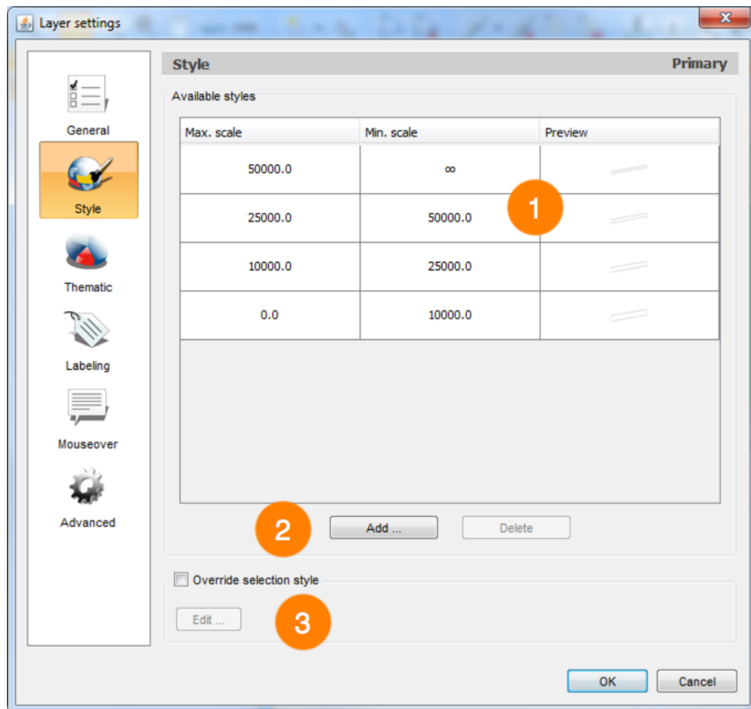
Interface for managing layer styles
