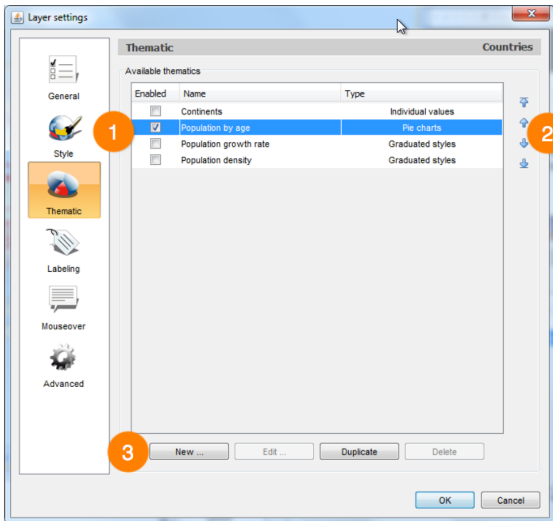
Thematic management interface
