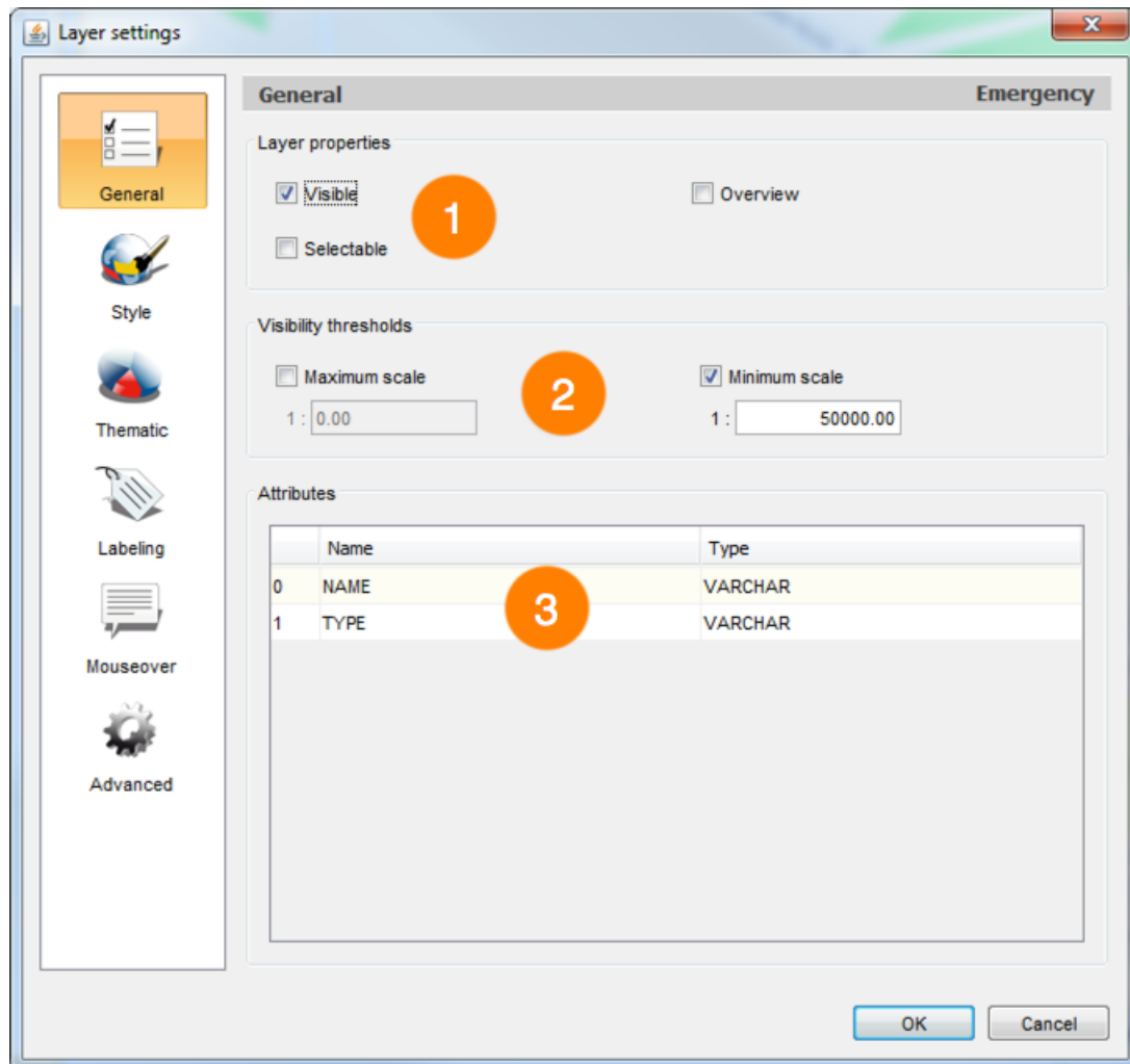
Interface for managing general layer settings
